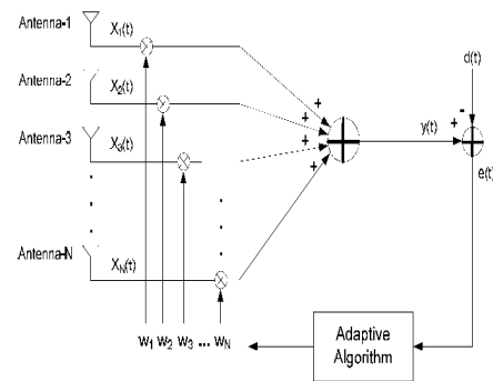
Fig.4 Adaptive beam-forming block diagram
