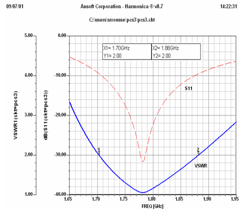
Fig.3 VSWR/Return Loss
